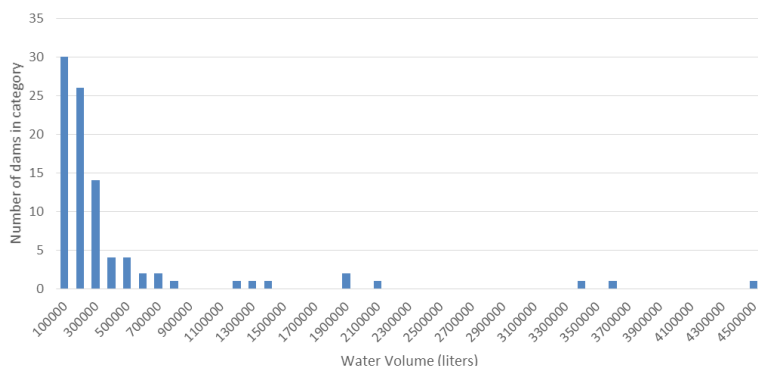
Figure 2. Calculated minimum available water volume of surveyed dams.
