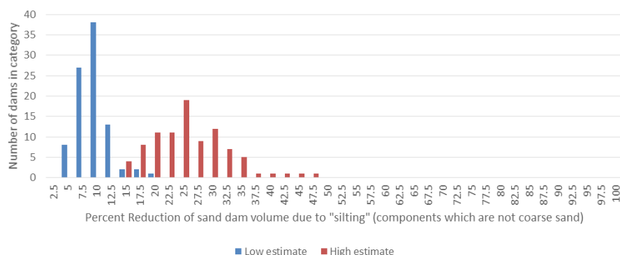
Figure 3 Siltation effects on calculated sand dam water volumes, based on low and high specific yield estimates.
