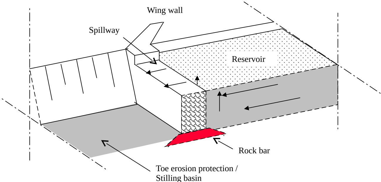
Figure 2.2: Principle of a sand-storage dam
